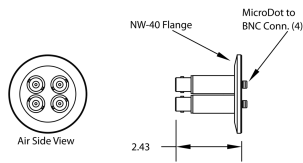
NW-40 Flange 4 MicroDot to BNC Conn. Part #200-040
